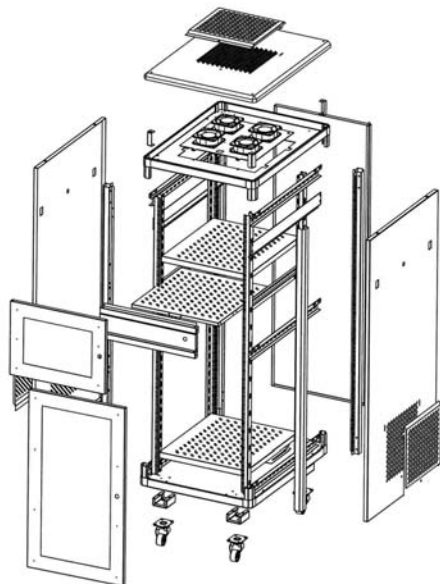
Explode View
