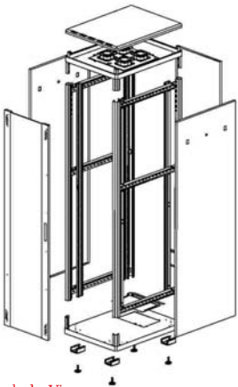
Explode View
