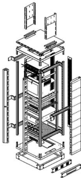
Explode View
